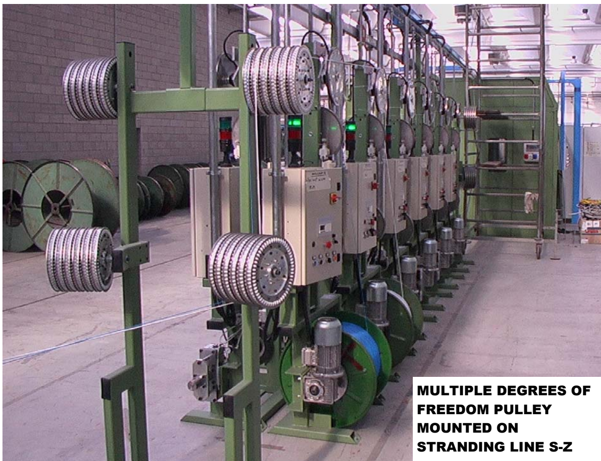
PULLEY ON VERTICAL PAY OFF
